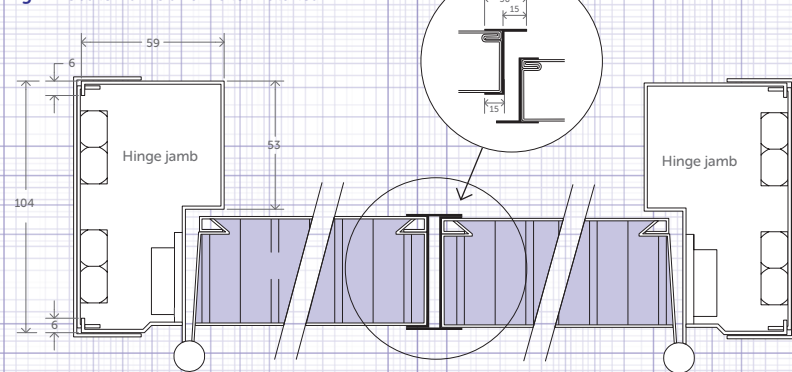
Fig. 2 Rebate frame and Dutch fold leaf
